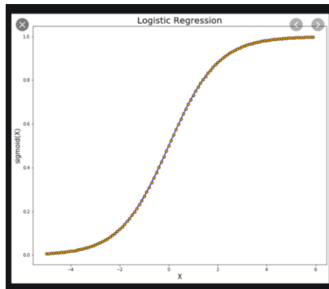
Fig.2 Logistic Regression
