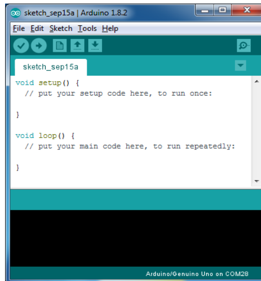
Figure 4: Arduino IDE
