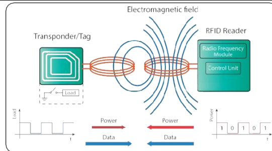
Figure 2: RFID Working Principles
