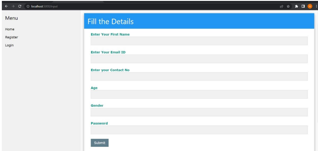
Fig. 1: Registration Page
