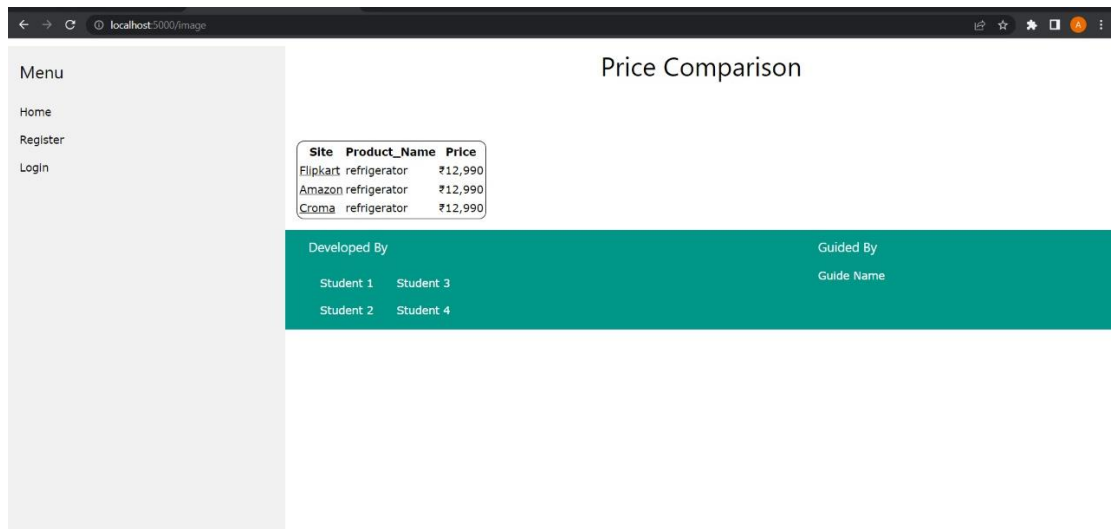
Fig. 4: Comparison Page
