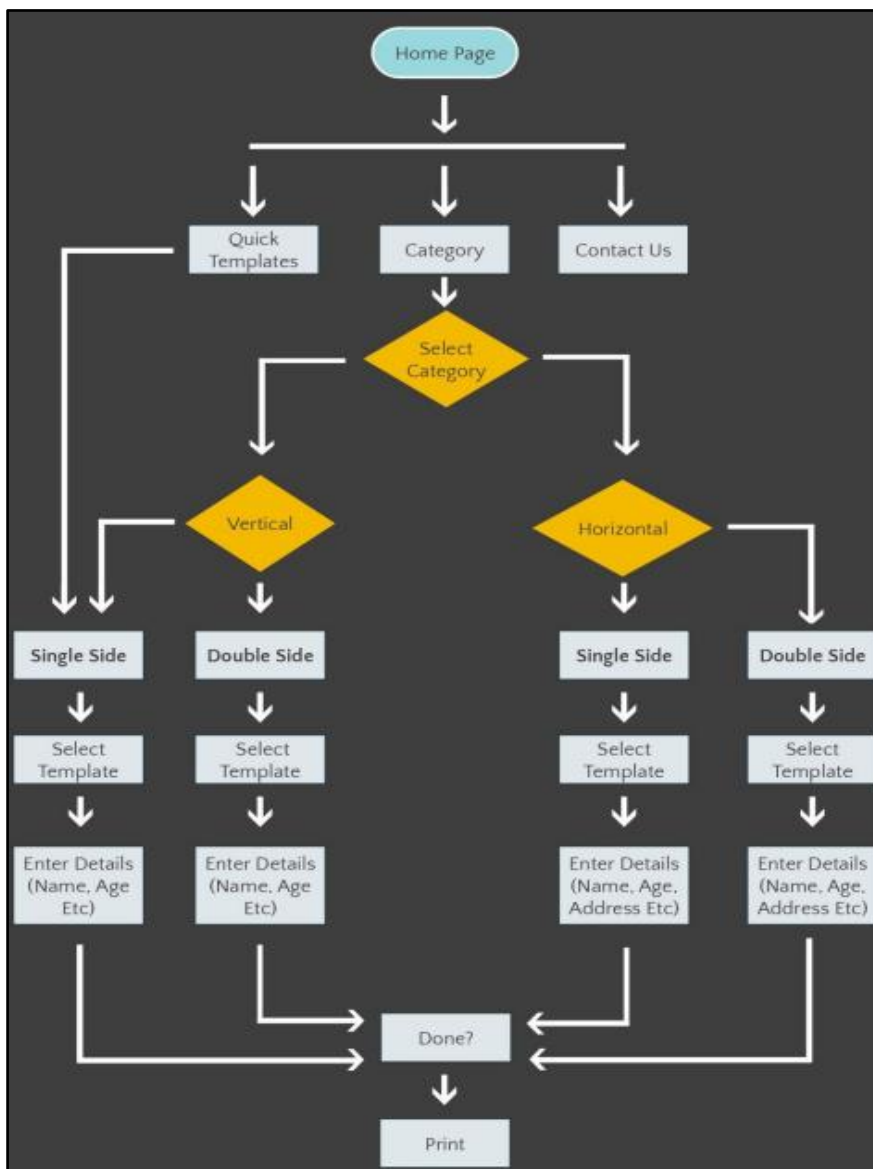
Figure 1: The proposed flow of the project
