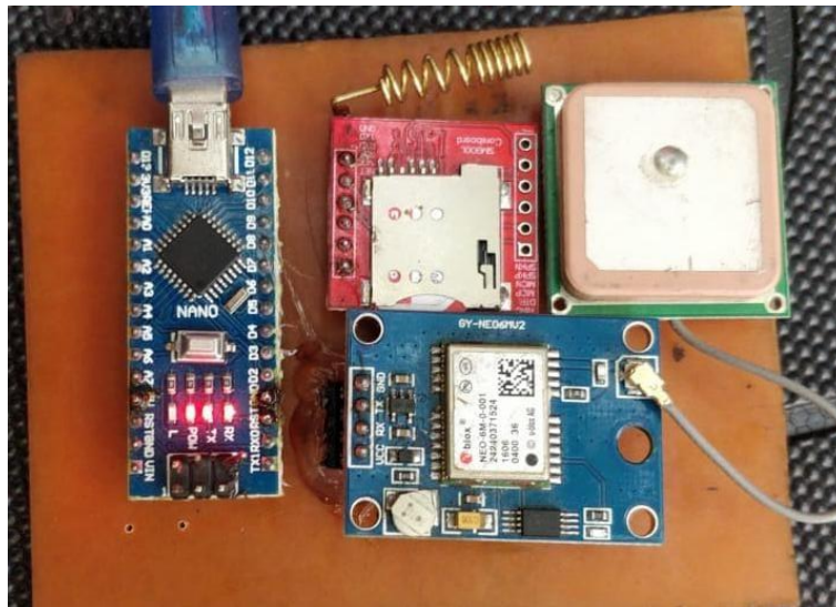
Fig: Snapshot of hardware of smart stick circuit
