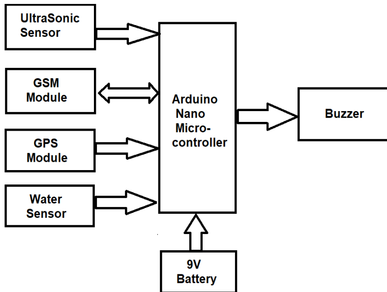
Fig: Block digram of Smart Stick
