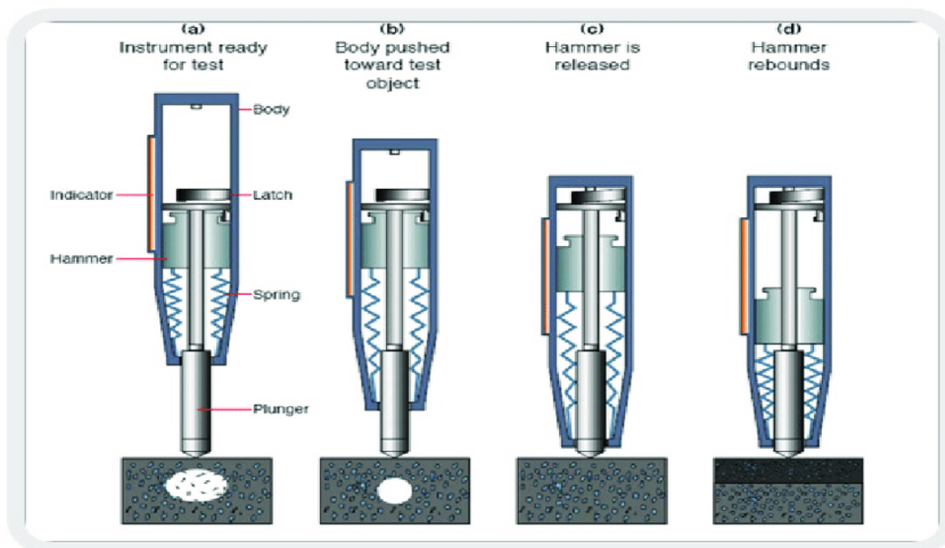
Fig. Rebound Hammer Test
