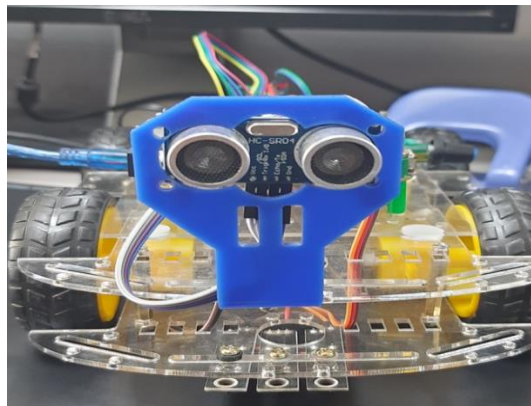
Fig. 2. Ultrasonic Sensor
