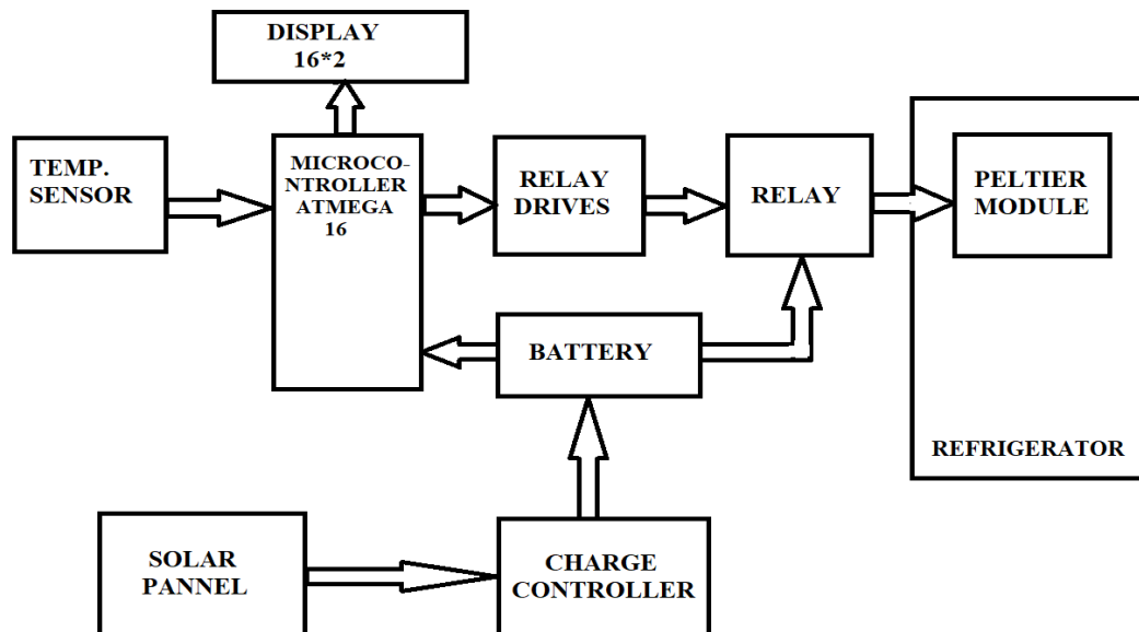
Fig-1: Block Diagram Solar Based Refrigeration System
