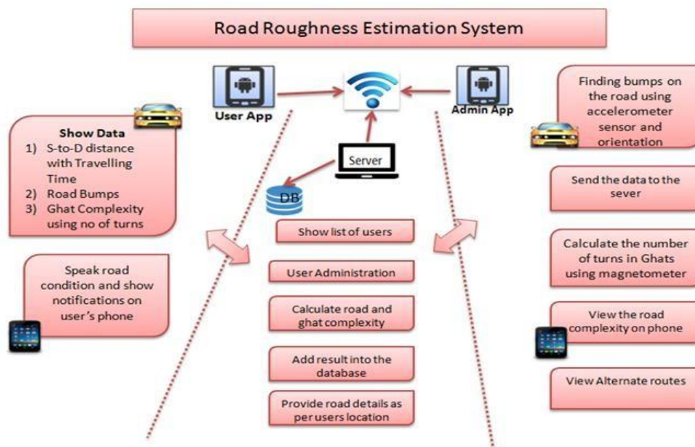
Fig.-1: Road Roughness Estimation System.
