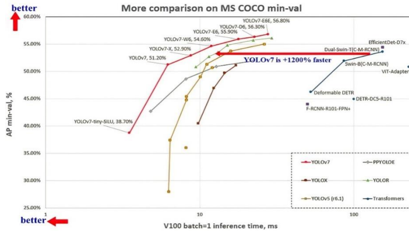
Fig 2 . Performance comparison of YOLOv7 vs. YOLOR vs. YOLOv5 vs. Vit transformers (source [6])
